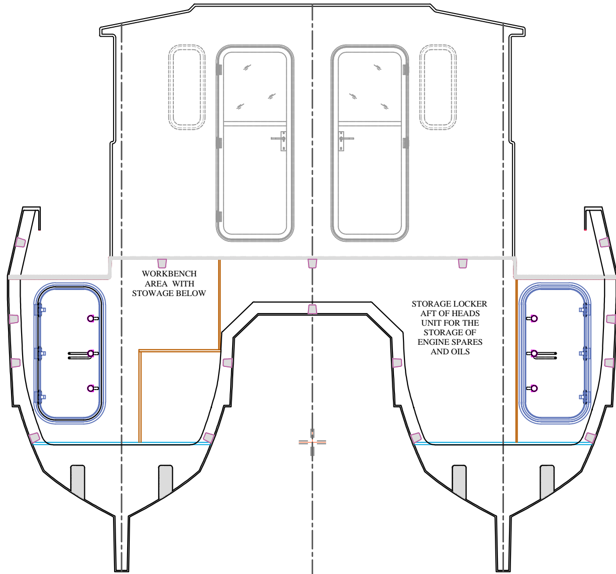
STATION 16 LOOKING AFT
