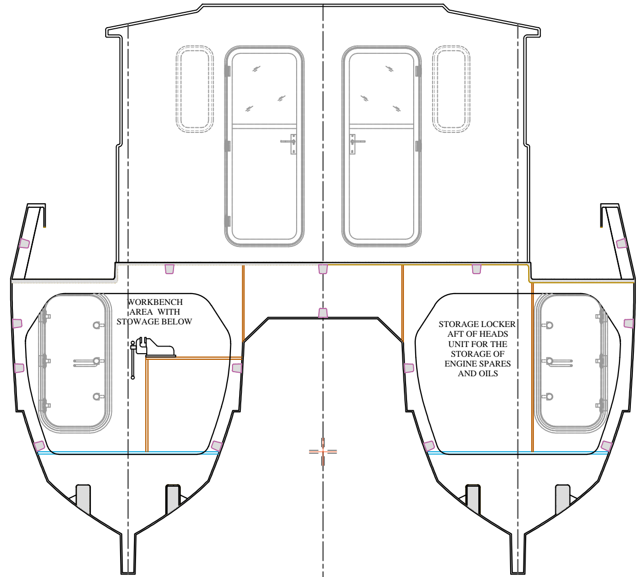
STATION 14 LOOKING AFT
