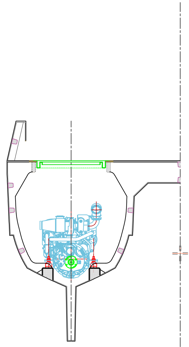
STATION 21 LOOKING AFT
