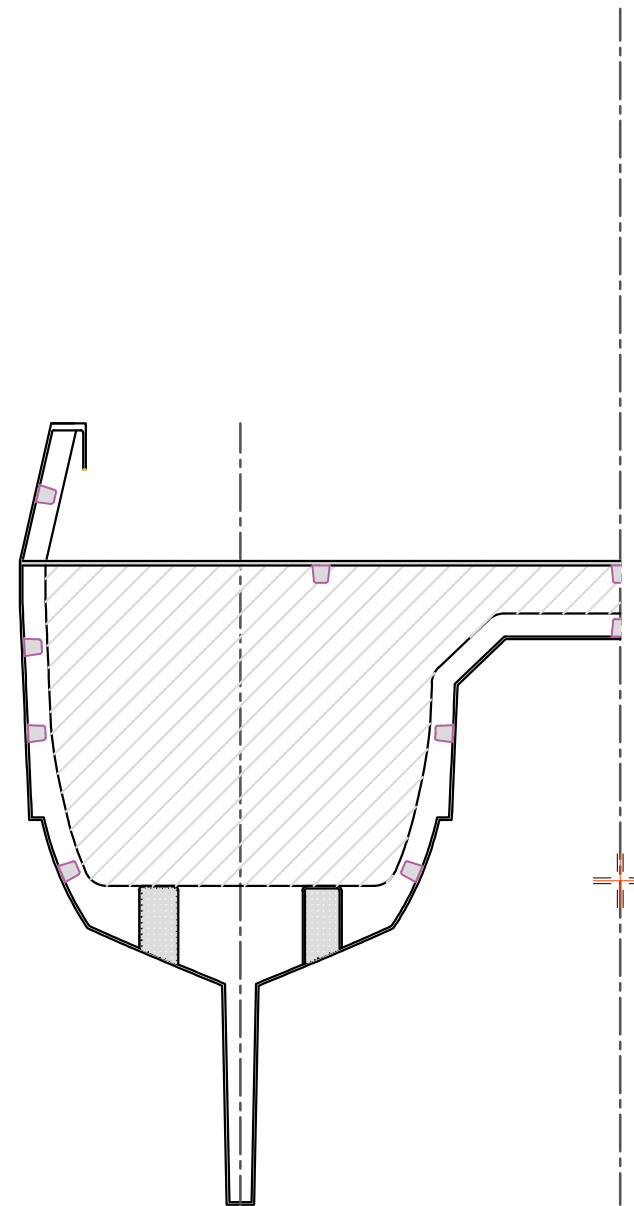
STATION 24 LOOKING AFT
