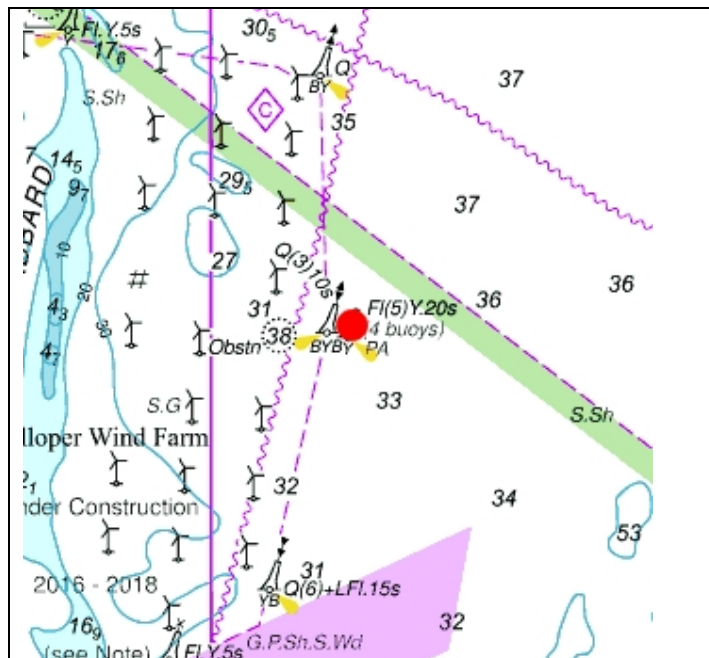
Fig. 3: Waverider Buoy Location West Gabbard
